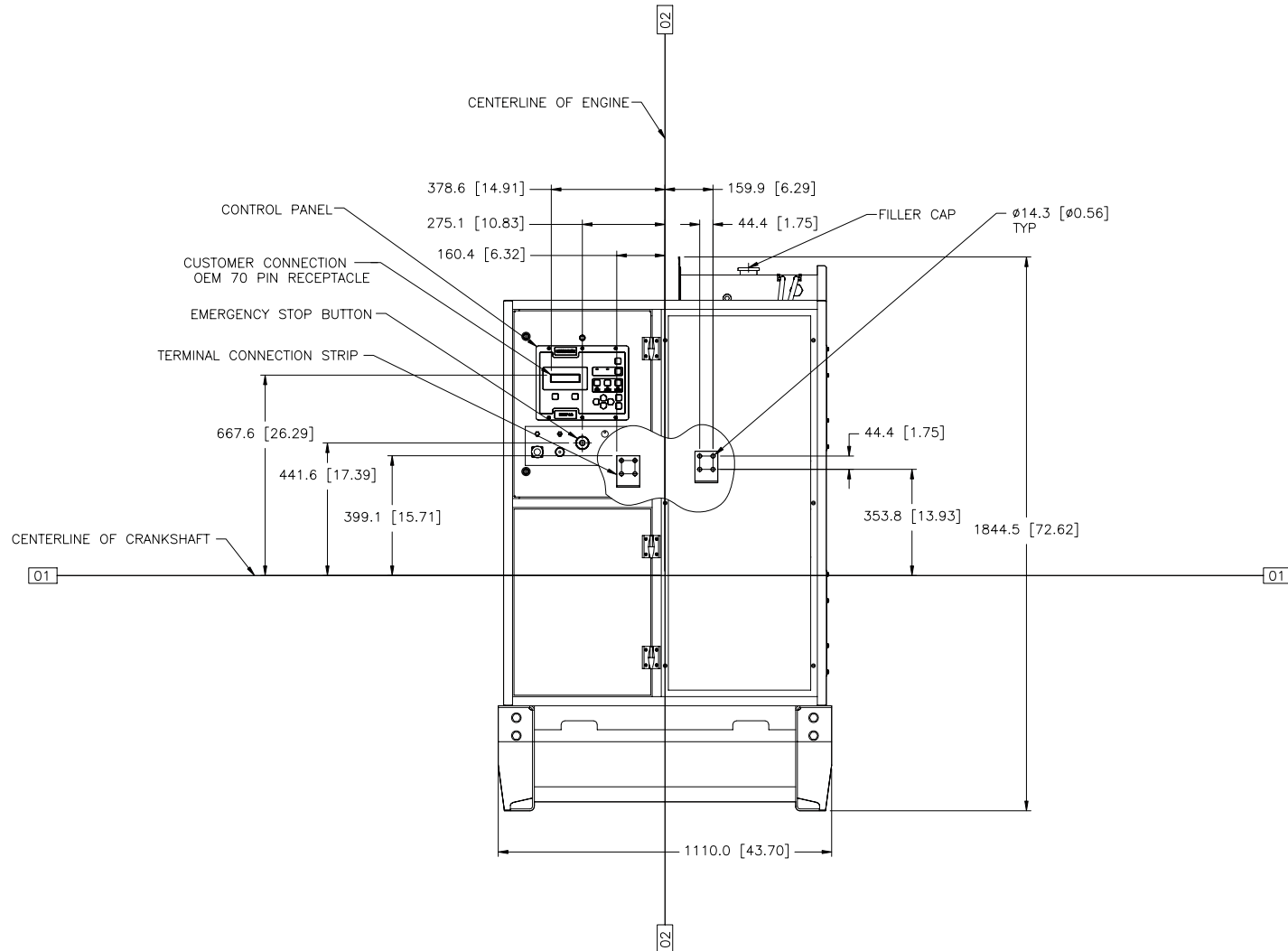
CAT C9 PACKAGE GENSET DWG# 277-8059 CHG 06 METRIC [INCH] REAR VIEW DK-2065 CHG 15 SHOWN
